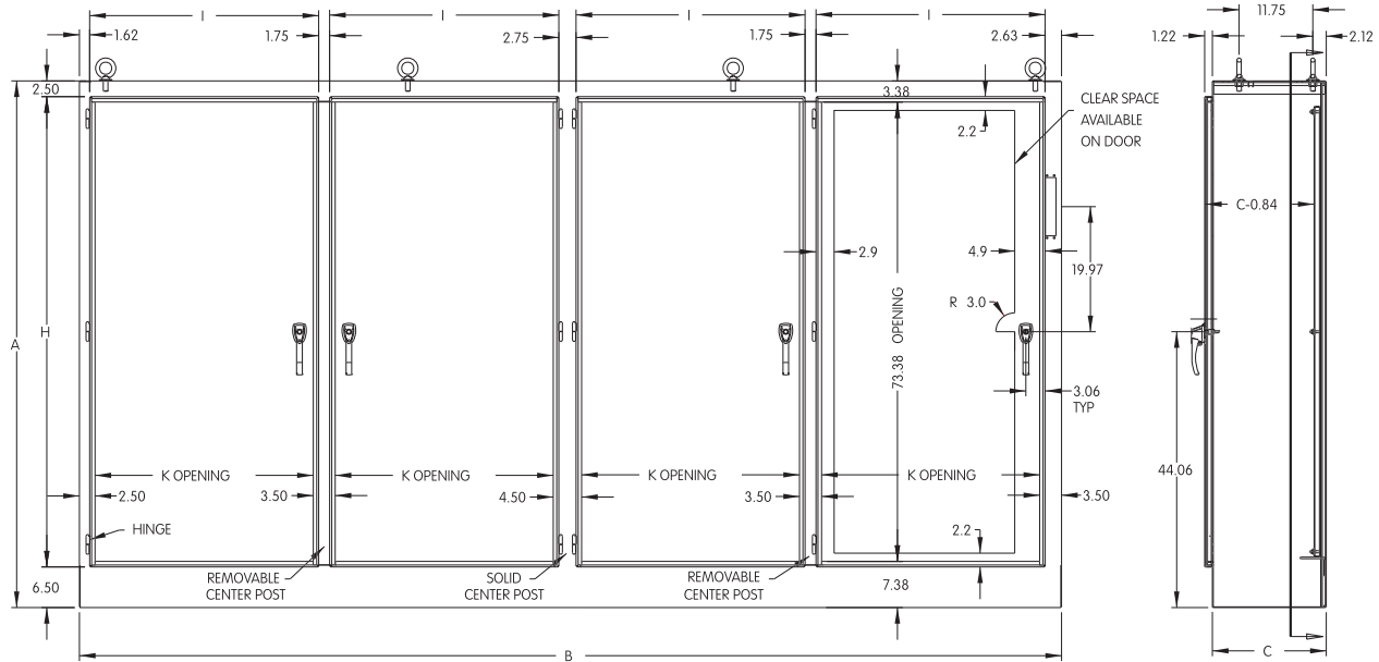
Front View
